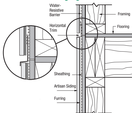
Figure 13 Bridging Floors
