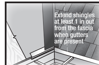
Figure 12 Valley/Shingle Extension
