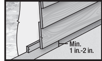
Figure 11 Mortar/Masonry
