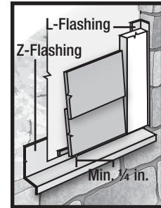
Figure 11 Mortar/Masonry
